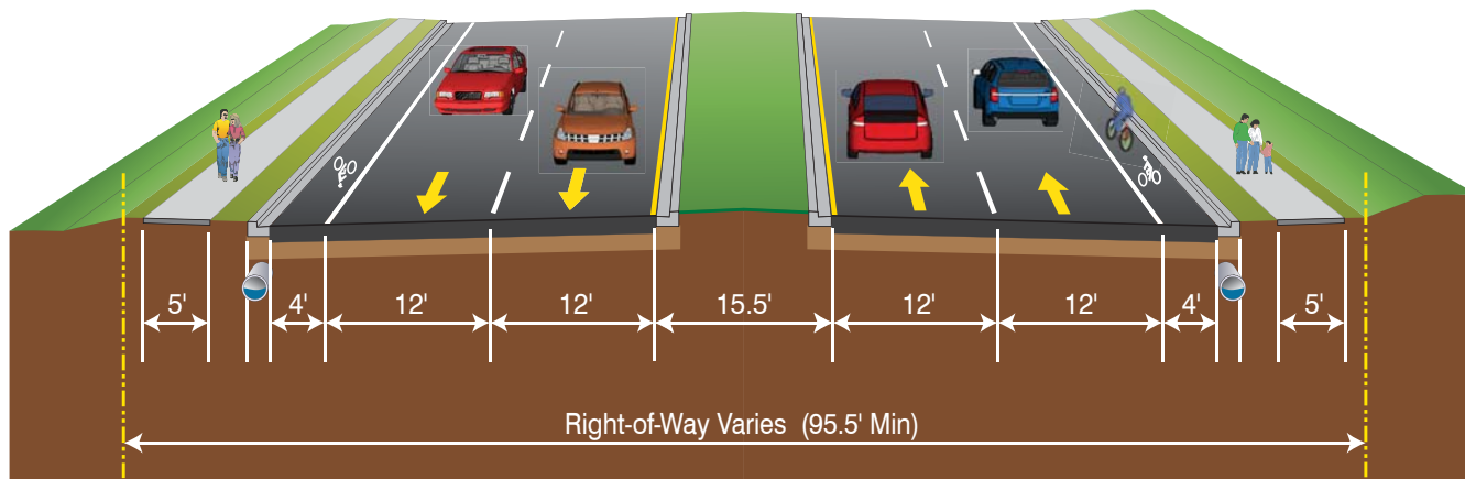
4-Lane Modified Urban Typical Section Design Speed 45 M.P.H.
