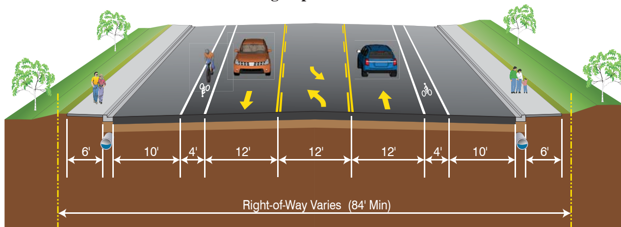
3-Lane Urban Typical Section with On-Street Parking (Downtown Malabar) Design Speed 45 M.P.H.
