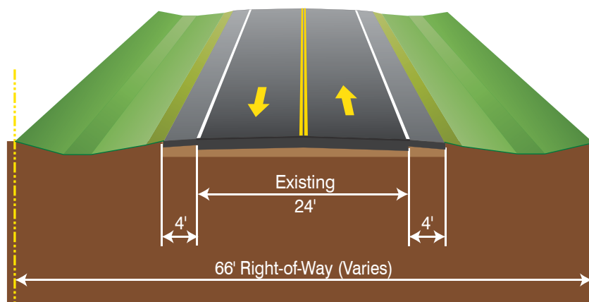
Existing Typical Section • From Enchanted Lakes to Marie Street (2.1 miles) Posted Speed 55 M.P.H.
