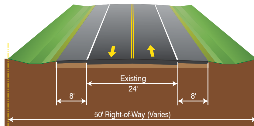
Existing Typical Section • From Marie Street to US 1 (.6 miles) Posted Speed 30 M.P.H.
