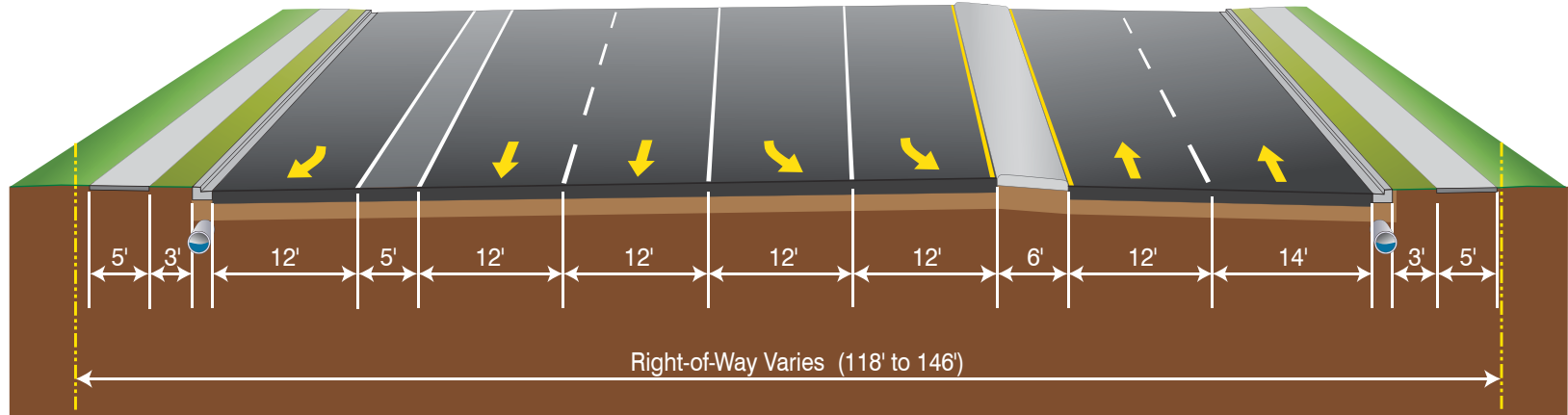
Existing Typical Section • From Babcock Street to Enterprise Avenue (.2 miles) Posted Speed 45 M.P.H.
