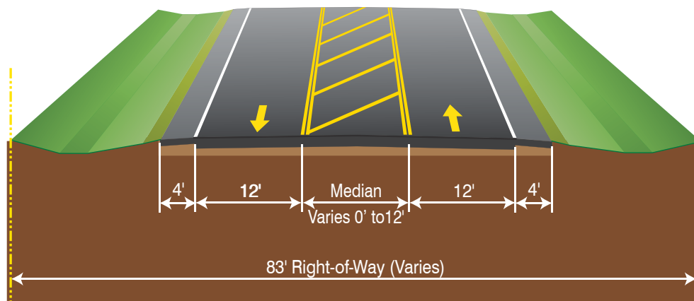
Existing Typical Section • From Enterprise Avenue to Enchanted Lakes (.8 miles) Posted Speed 45 M.P.H.
